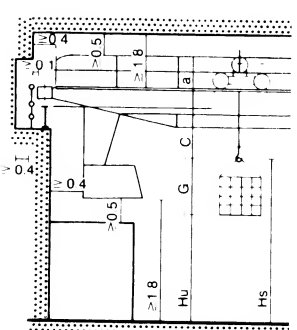
⑯ Gantry crane (safety dimensions)
